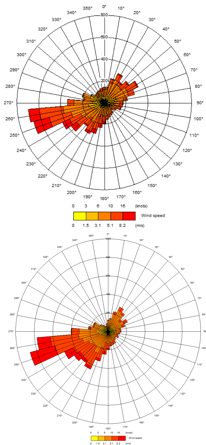
Figure 1.1: Year 2015 Wind Rose for Bristol Filton Airport
